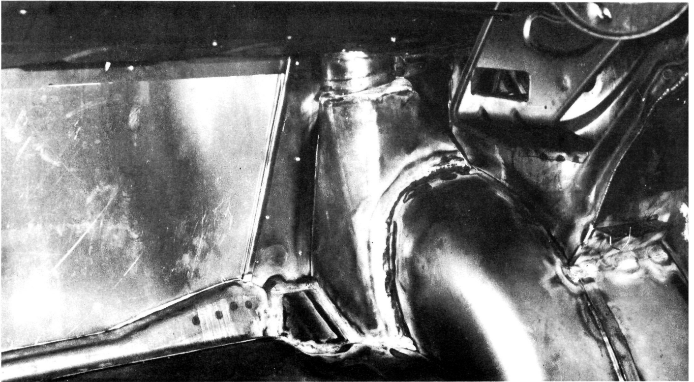
Works turret viewed from inside boot. Damper top nut access is from inside cockpit.
