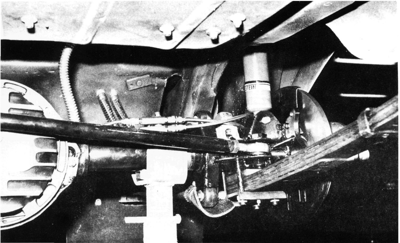
General suspension seen from below. Note panhard rod mounting.
