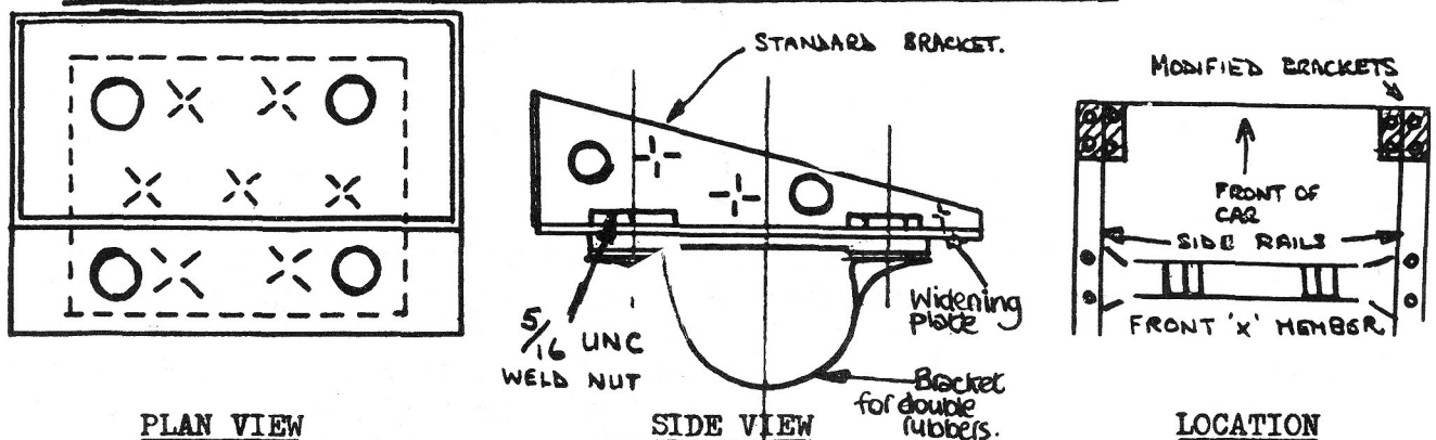
Double width anti-roll bar mounting drawings (not to scale)
